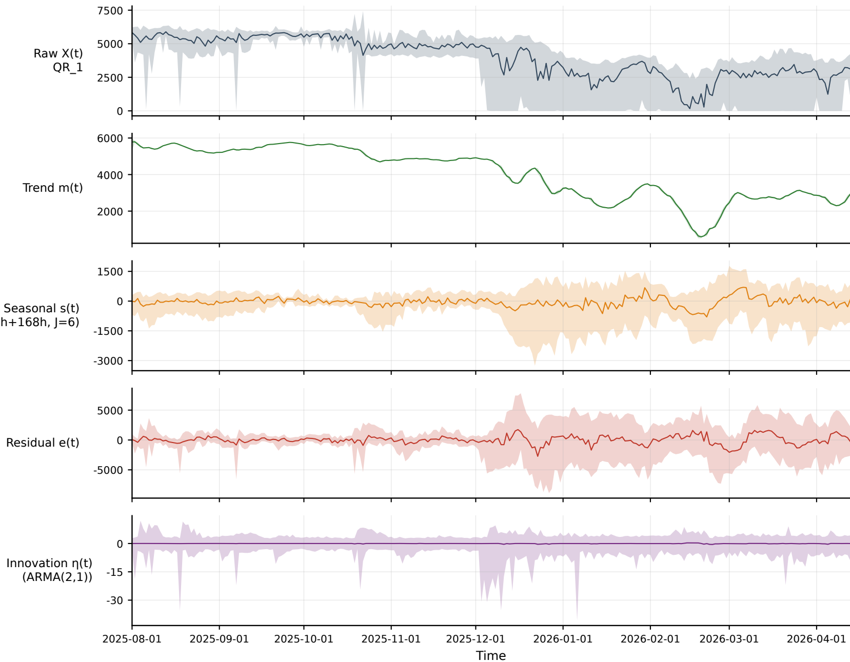
Full-span daily overview — QR_1 (recycle, min) [2025-08-01~2026-04-13]
